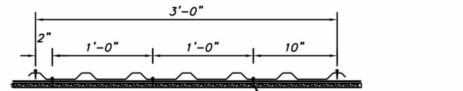
SCREW SPACING
