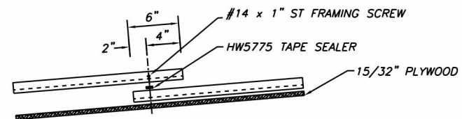
LATERAL PANEL LAP
